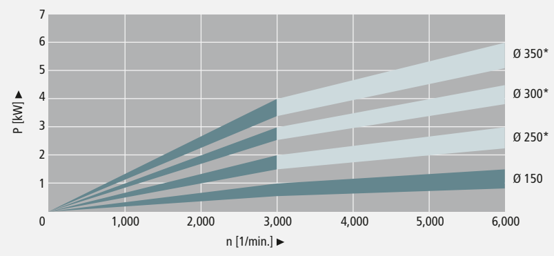
Power requirements for Wheel Brushes
